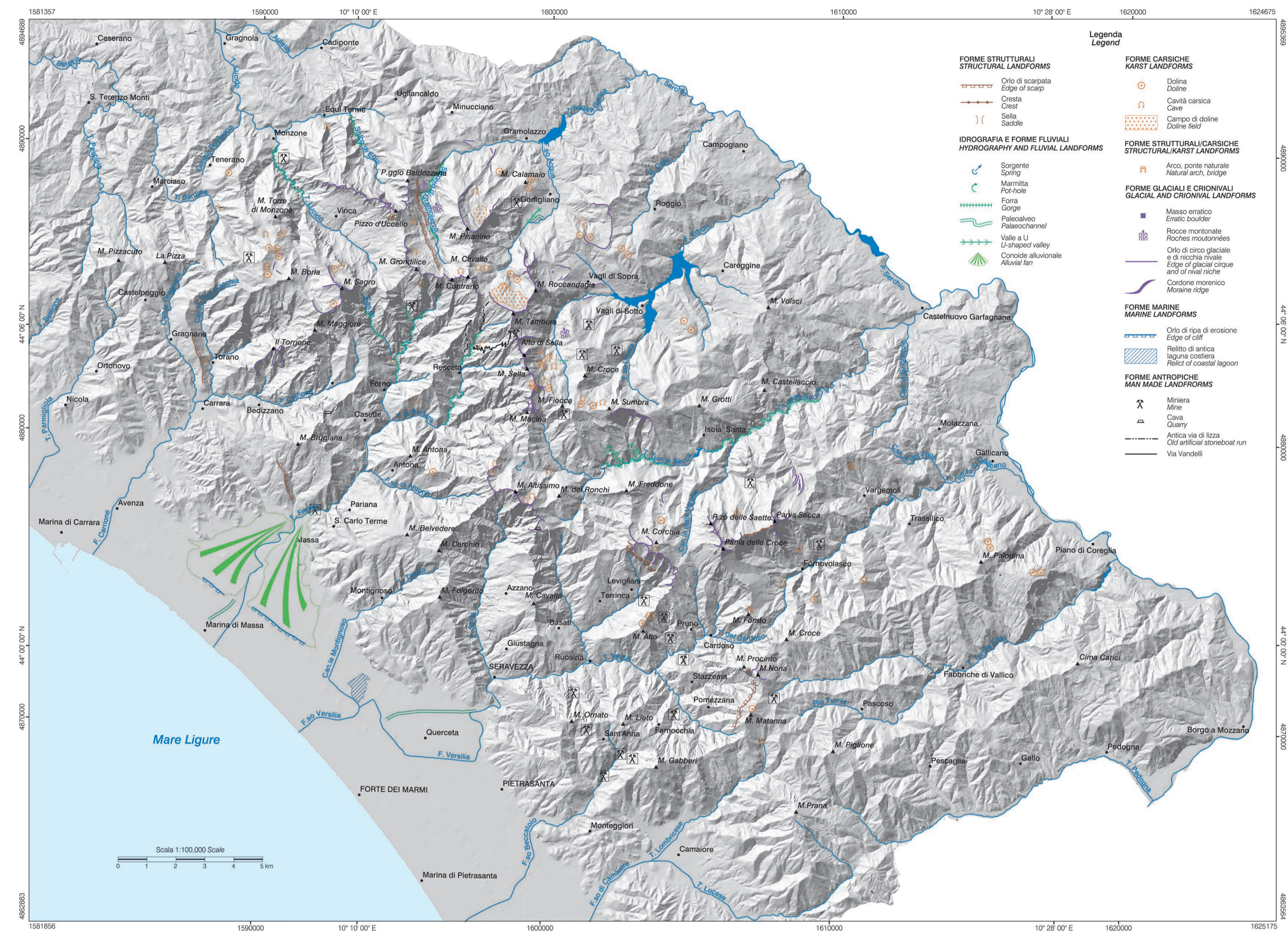
SCHEMA DELLE PRINCIPALI EMERGENZE GEOMORFOLOGICHE MAP OF SELECTED SITES OF GEOMORPHOLOGICAL SIGNIFICANCE
